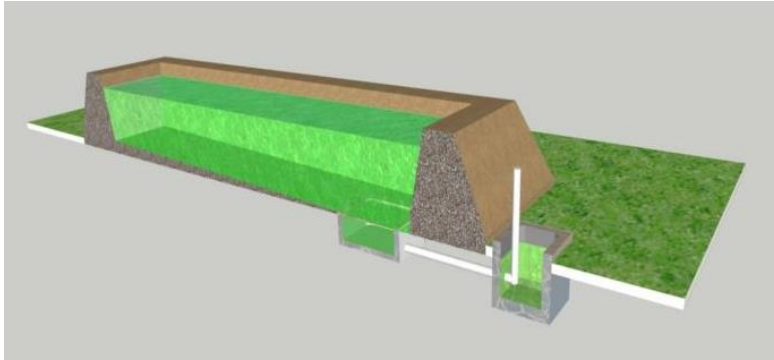
Figure.25: A schematic diagram for slope construction
