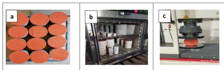
Figure 2. Shows: a) preparation of specimens filmed on both cross-sectional faces to impose CO 2 diffusion in one direction only; b) placing of specimens in the carbonation chamber; c) breaking of specimens by splitting to spray phenolphthalein.
