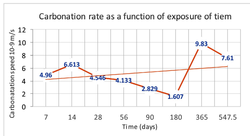
Figure 5. Carbonation rate as a function of exposure time.
