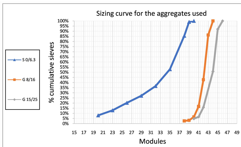
Figure 1. Sizing curve for the aggregates used.
