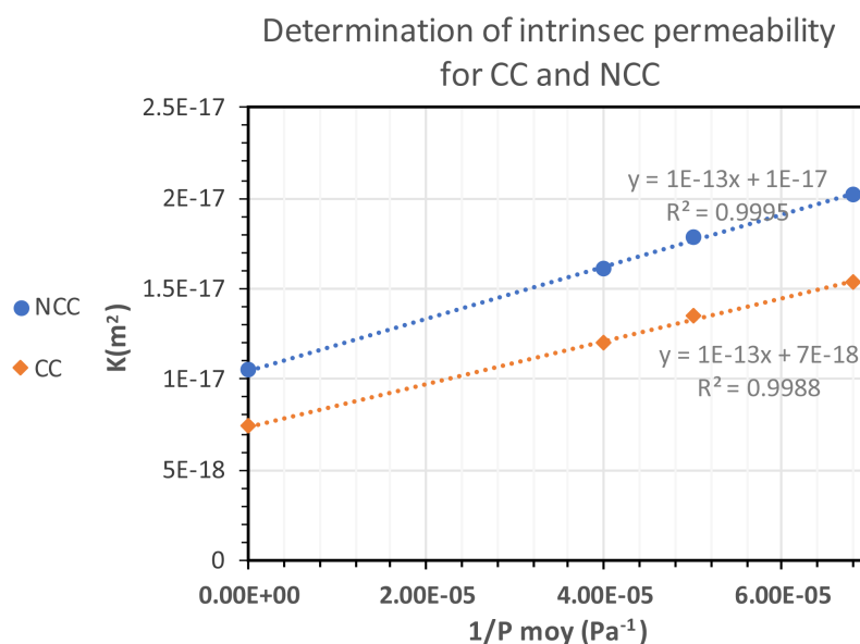
Figure 7. Determination of intrinsic permeability for CC and NCC.
