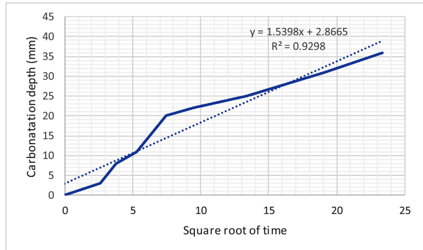
Figure 4. Carbonation depth as a function of the square root of time.
