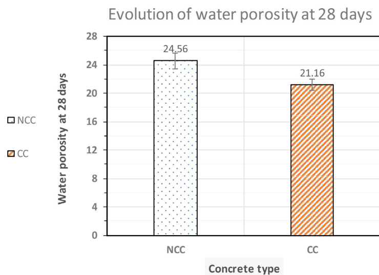
Figure 6. Evolution of porosity before and after carbonation.
